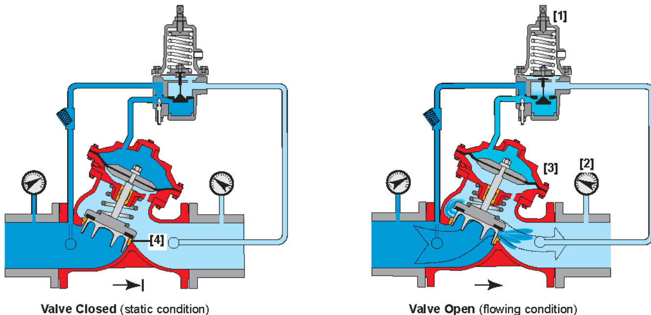
Figure 2: Operation Drawing
