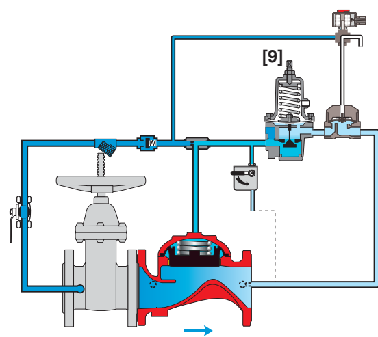
Valve Open (operating condition)
