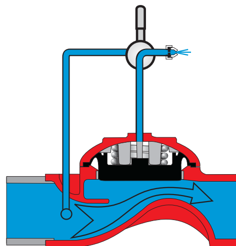
Valve Open
